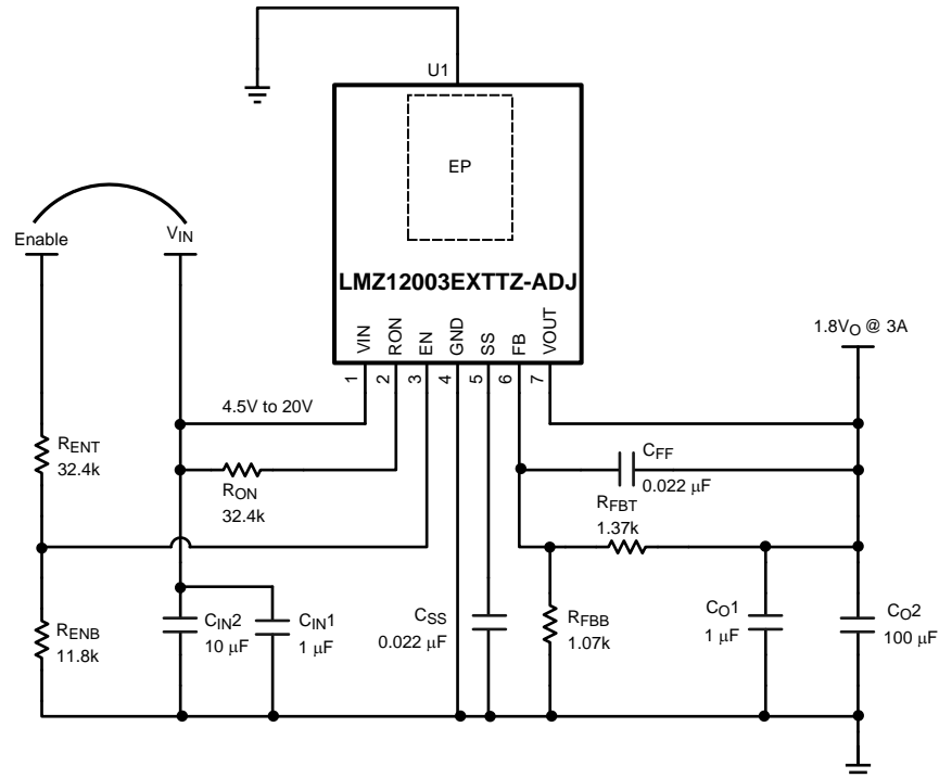
Figure 21. Evaluation Board Schematic Diagram
